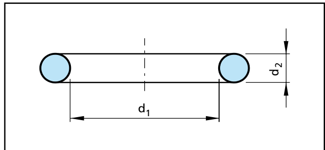
Figure 5 O-Ring dimensions
